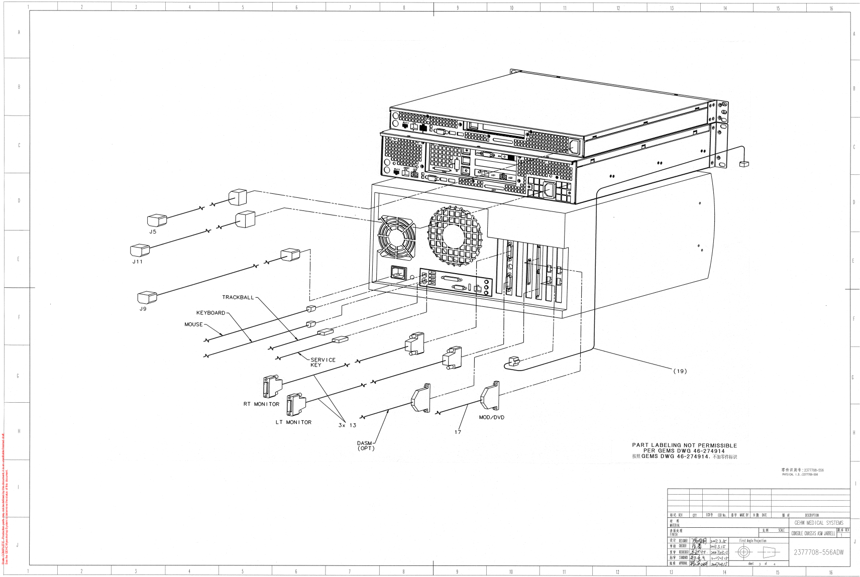
Figure 5-10 GRE CONSOLE,16slice MDAS and GDAS with XW8200 and 1IG, JARRELL (2377708-556, sheet 3, rev 1)
