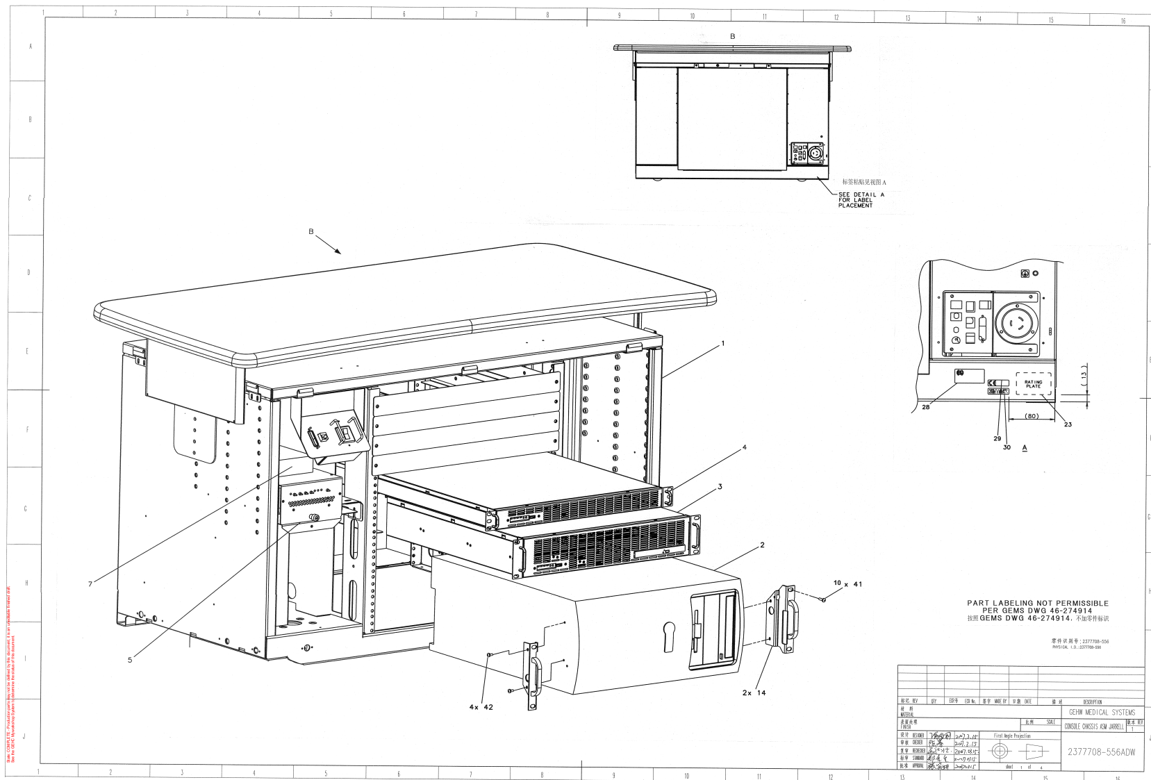
Figure 5-8 GRE CONSOLE, 16slice MDAS and GDAS with XW8200 and 1IG, JARRELL (2377708-556, sheet 1, rev 1)
