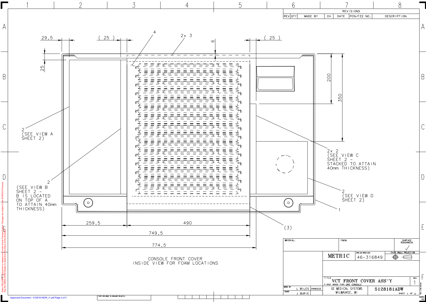
Figure 5-7 Cover Assy - Console Front (5128181 Sheet 1, Rev 1)
