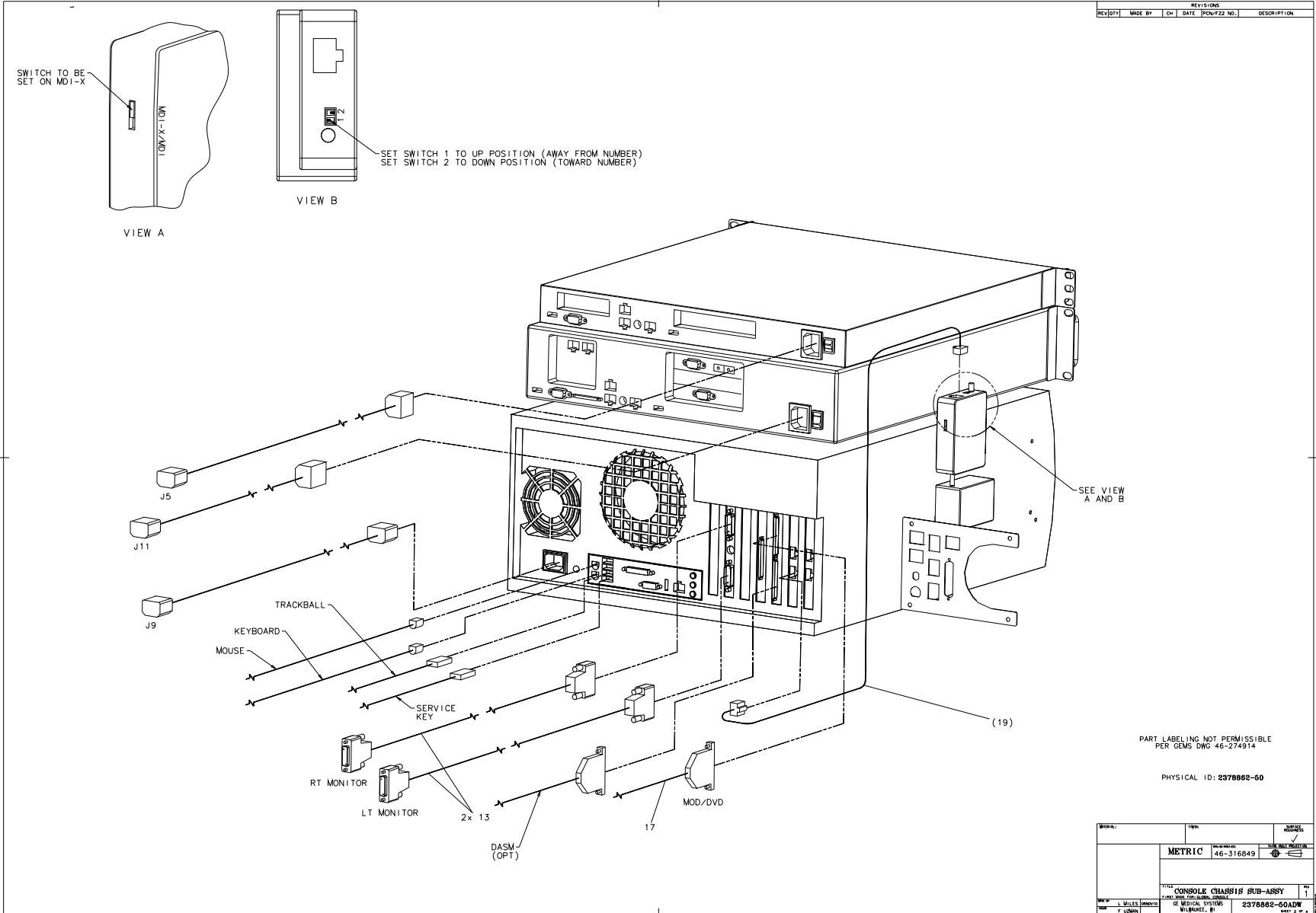
Figure 5-3 GOC4 (2378862-56, sheet 3, rev 1)
