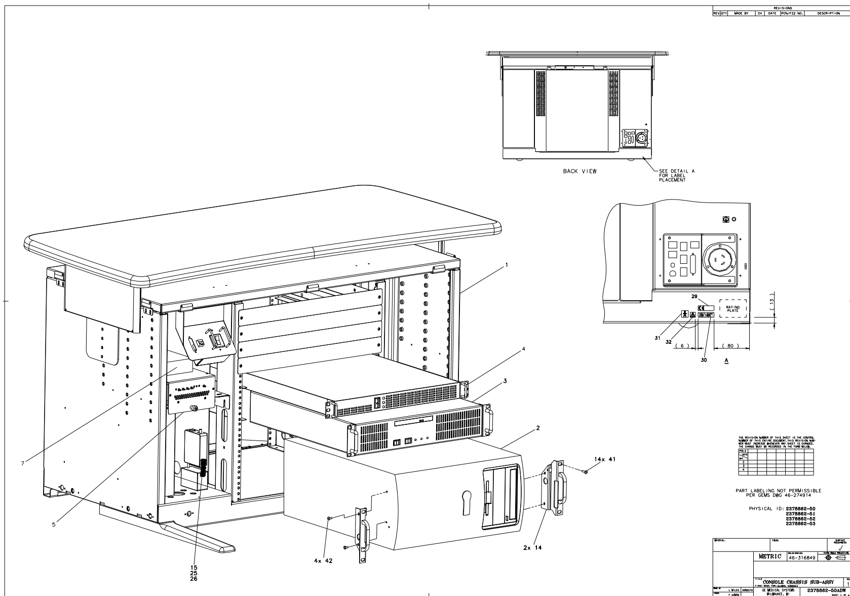
Figure 5-1 GOC4 (2378862-56, sheet 1, rev 1)
