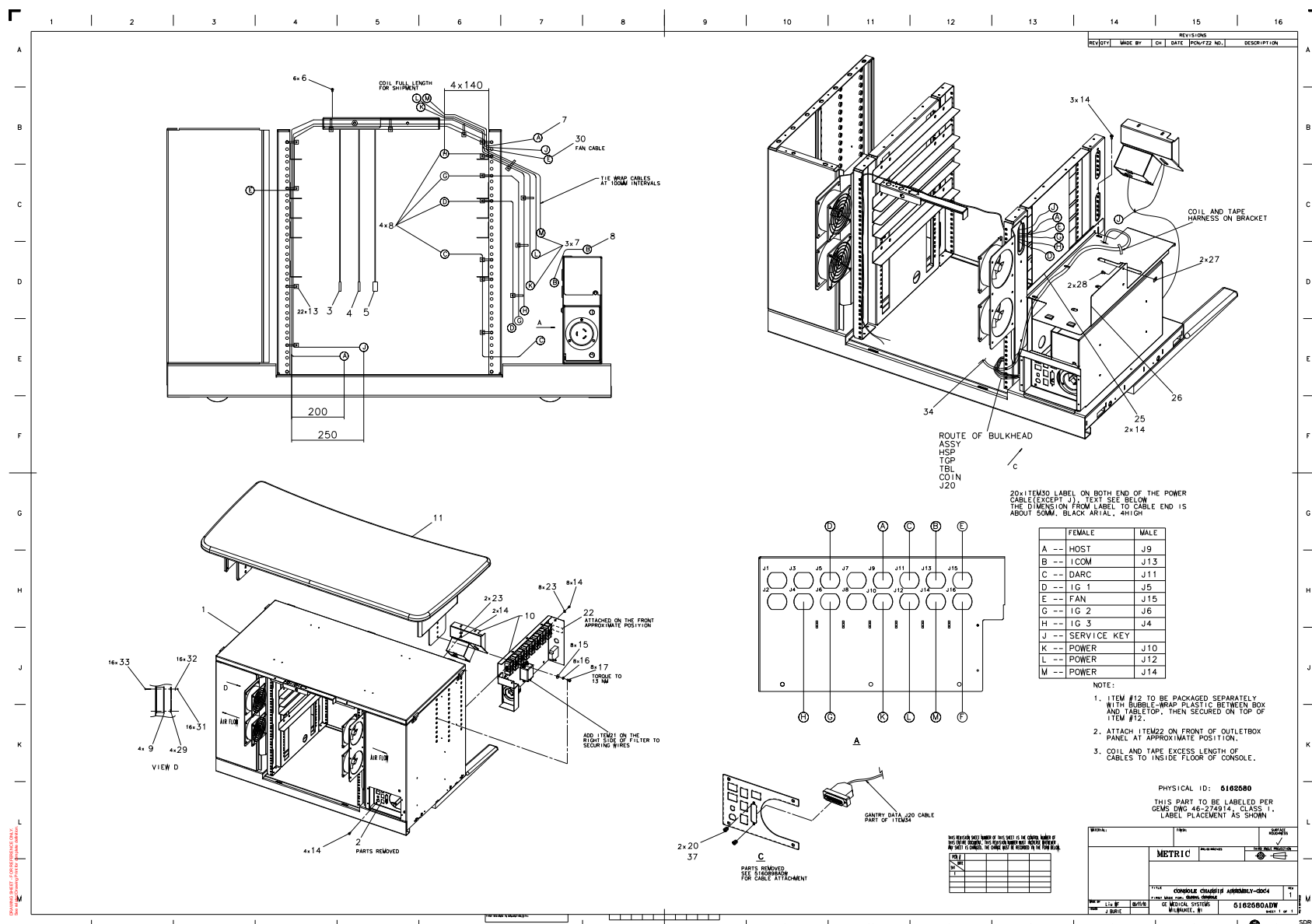
Figure 5-5 New GOC4 Chassis (5162580 Sheet 1, Rev 1)
