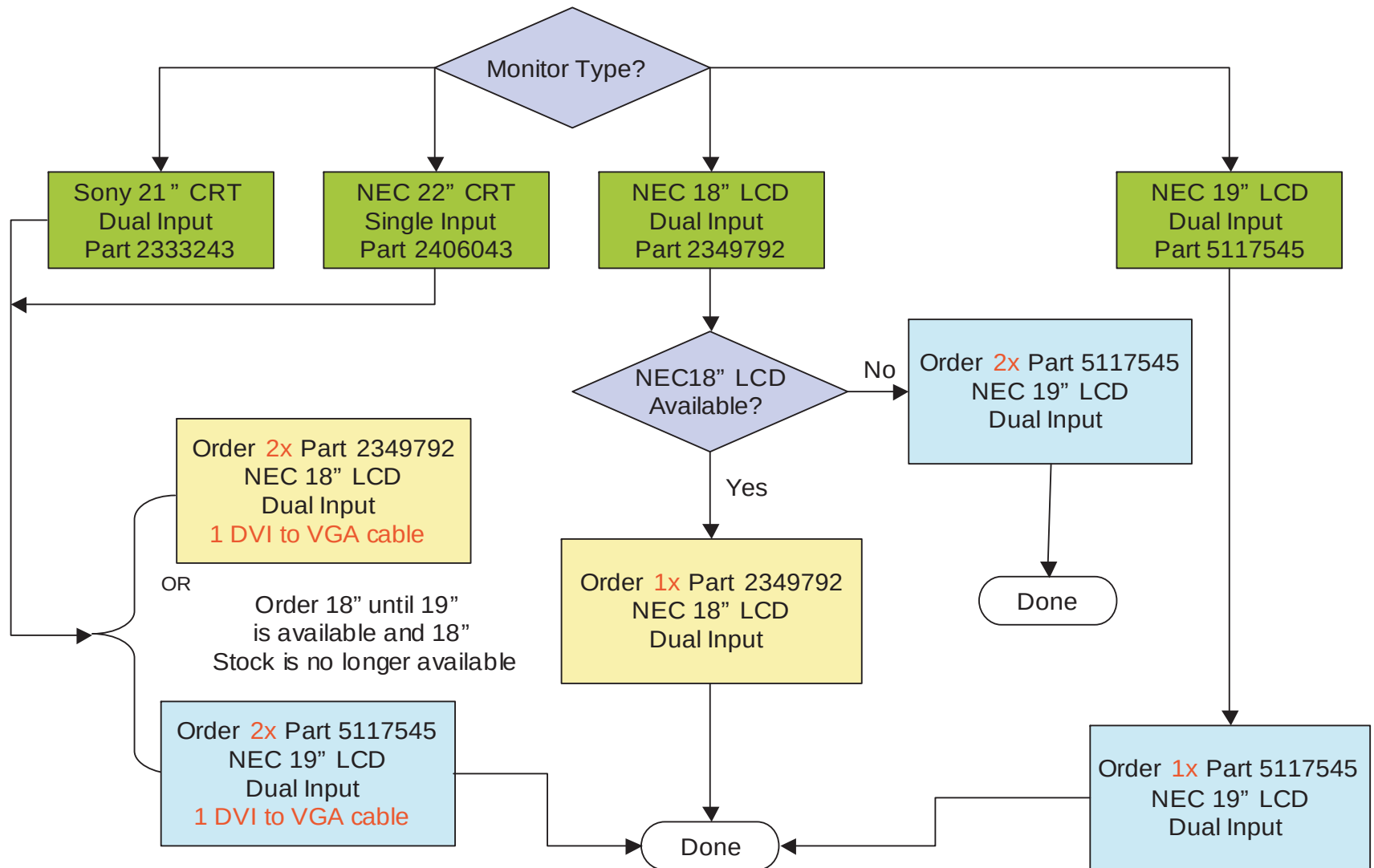
Figure 5-13 Monitor Selection Flowchart
