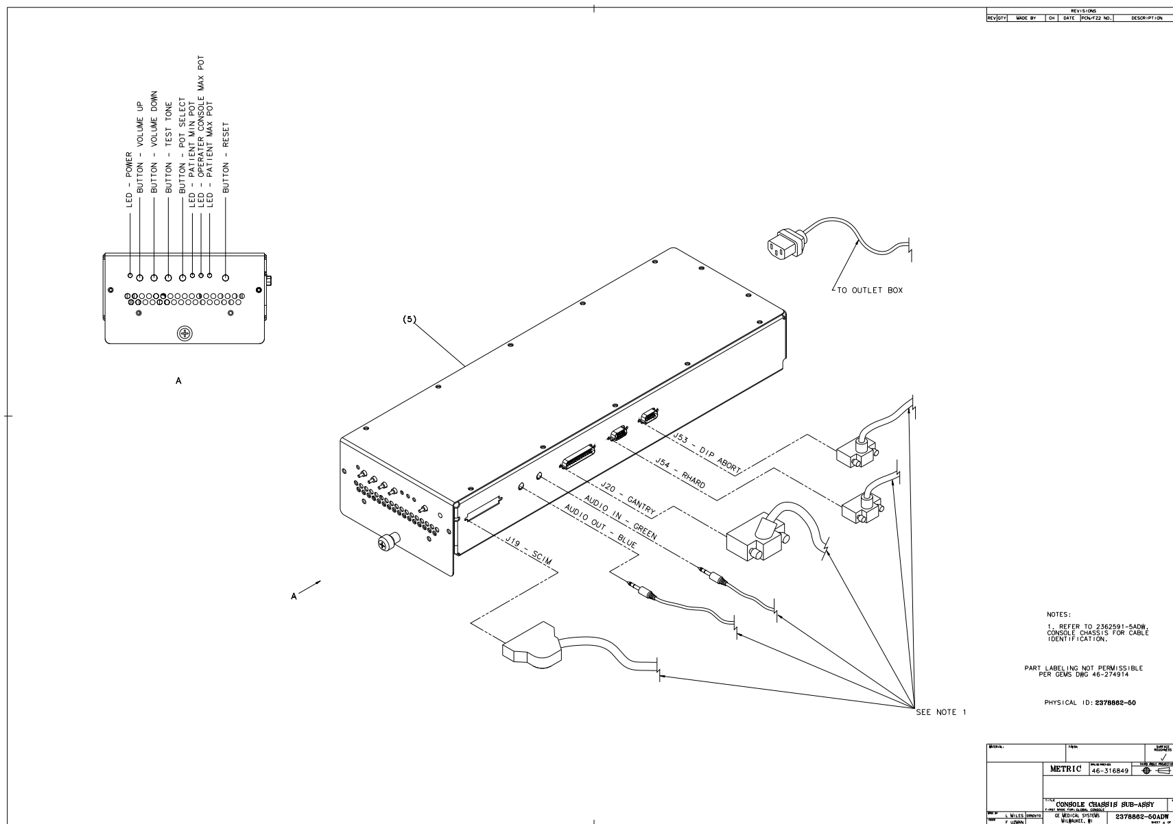
Figure 5-4 GOC4 (2378862-56, sheet 4, rev 1)
